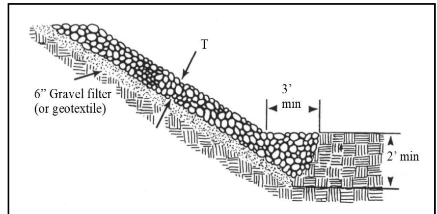
Typical riprap slope protection detail
