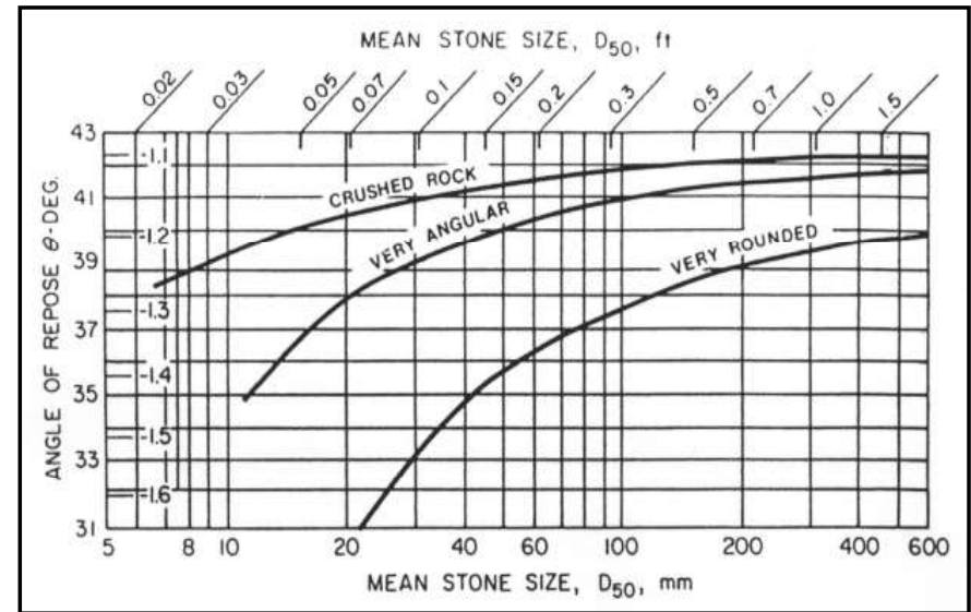
Angle of repose of riprap stones (FHWA)
