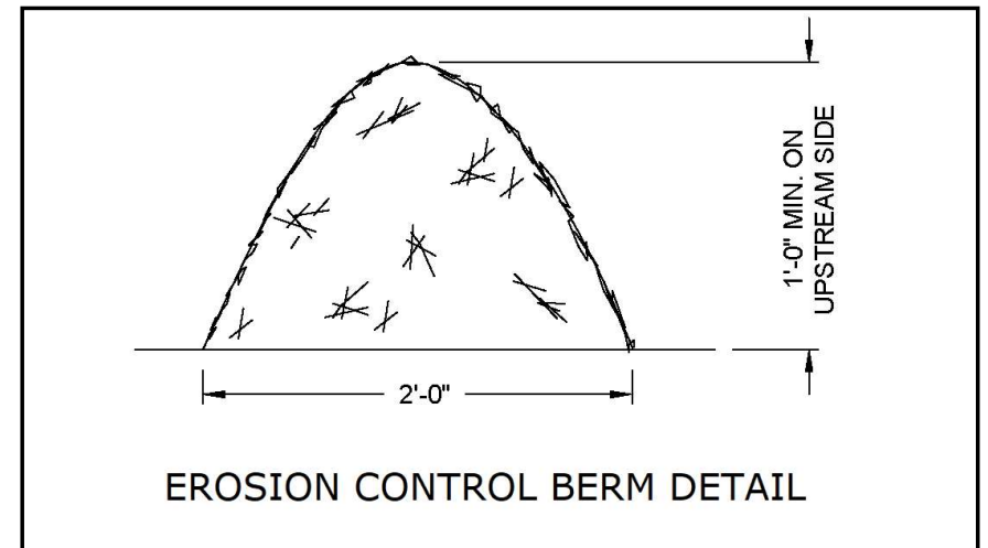
The erosion control berm above is allowing for both ponding and filtering of stormwater.
